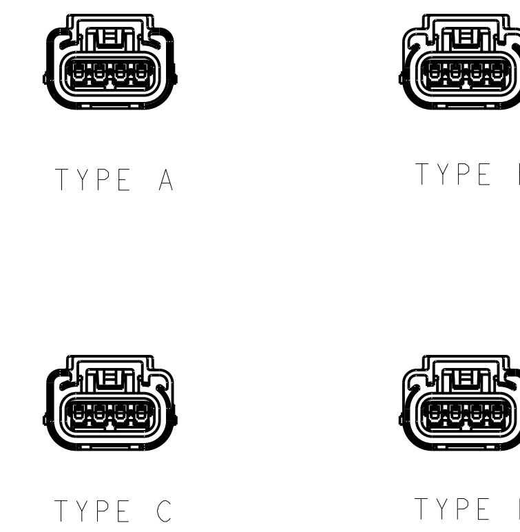
POLARIZATION OPTIONS SCALE 1:1
