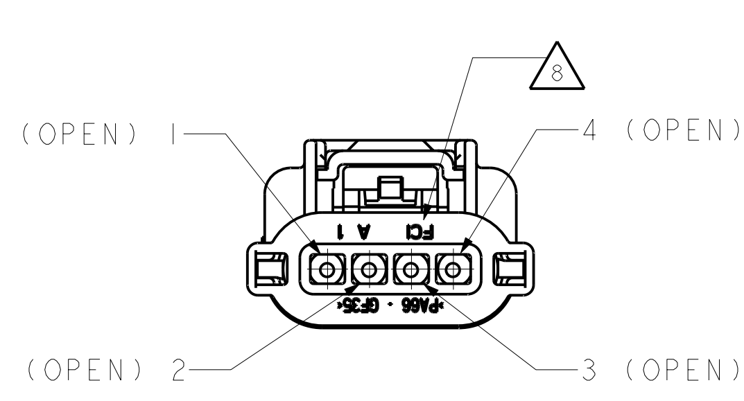
SECTION A-A SEALED ASSEMBLY VIEW FOR REFERENCE ONLY
