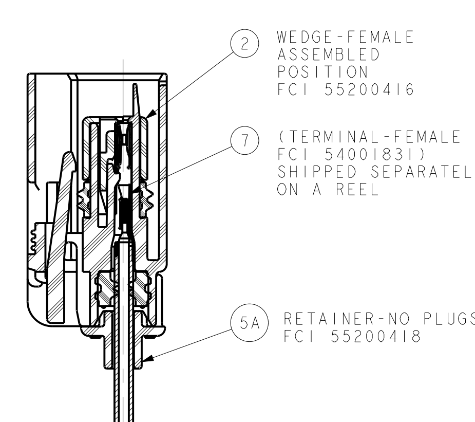
SECTION B-B SEALED ASSEMBLY VIEW FOR REFERENCE ONLY
